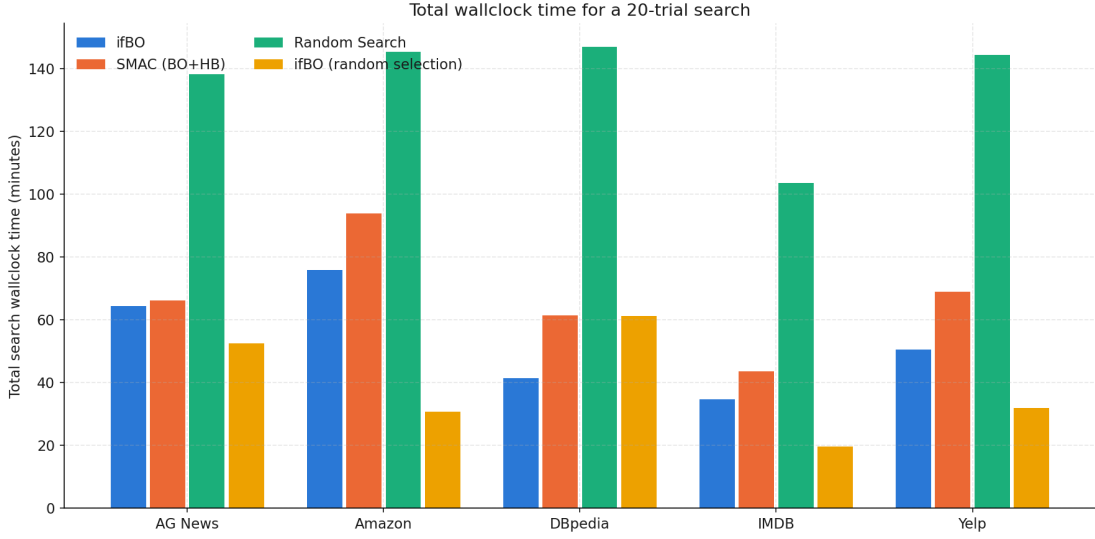
Figure 6: Total wall-clock time per dataset and method.
